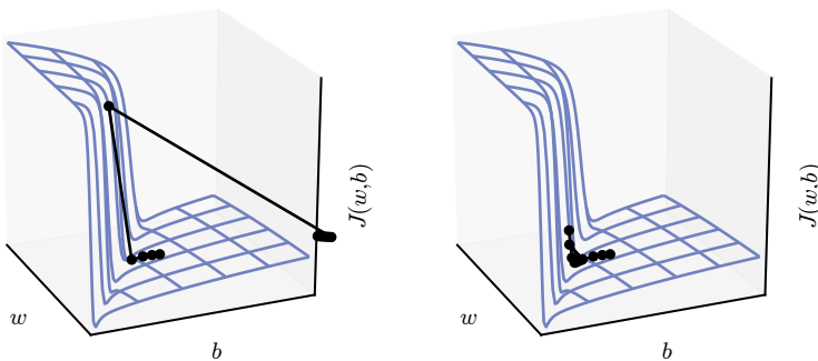
Figure 10.17: Example of the effect of gradient clipping in a recurrent network with two parameters w and b . Gradient clipping can make gradient descent perform more reasonably in the vicinity of extremely steep cliffs. These steep cliffs commonly occur in recurrent networks near where a recurrent network behaves approximately linearly. The cliff is exponentially steep in the number of time steps because the weight matrix is multiplied by itself once for each time step. (Left) Gradient descent without gradient clipping overshoots the bottom of this small ravine, then receives a very large gradient from the cliff face. The large gradient catastrophically propels the parameters outside the axes of the plot. (Right) Gradient descent with gradient clipping has a more moderate reaction to the cliff. While it does ascend the cliff face, the step size is restricted so that it cannot be propelled away from the steep region near the solution. Figure adapted with permission from Pascanu et al. (2013).
