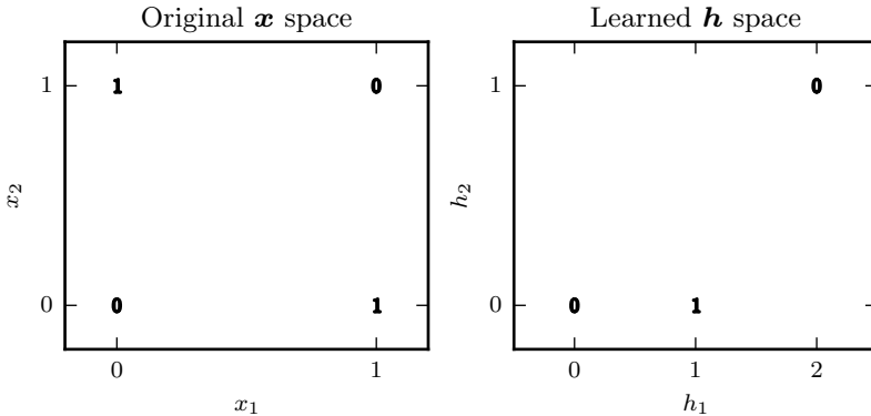
Figure 6.1: Solving the XOR problem by learning a representation. The bold numbers printed on the plot indicate the value that the learned function must output at each point. ( Left ) A linear model applied directly to the original input cannot implement the XOR function. When x_1 = 0 , the model’s output must increase as x_2 increases. When x_1 = 1 , the model’s output must decrease as x_2 increases. A linear model must apply a fixed coefficient w_2 to x_2 . The linear model therefore cannot use the value of x_1 to change the coefficient on x_2 and cannot solve this problem. ( Right ) In the transformed space represented by the features extracted by a neural network, a linear model can now solve the problem. In our example solution, the two points that must have output 1 have been collapsed into a single point in feature space. In other words, the nonlinear features have mapped both \mathbf{x} = [1, 0]^\top and \mathbf{x} = [0, 1]^\top to a single point in feature space, \mathbf{h} = [1, 0]^\top . The linear model can now describe the function as increasing in h_1 and decreasing in h_2 . In this example, the motivation for learning the feature space is only to make the model capacity greater so that it can fit the training set. In more realistic applications, learned representations can also help the model to generalize.
