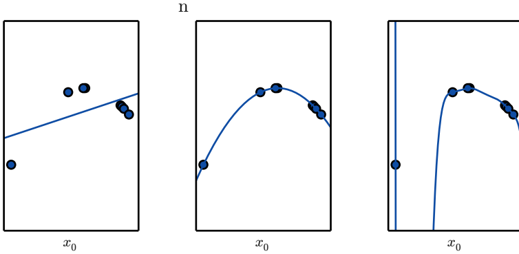
Figure 5.2: We fit three models to this example training set. The training data was generated synthetically, by randomly sampling x values and choosing y deterministically by evaluating a quadratic function. (Left) A linear function fit to the data suffers from underfitting—it cannot capture the curvature that is present in the data. (Center) A quadratic function fit to the data generalizes well to unseen points. It does not suffer from a significant amount of overfitting or underfitting. (Right) A polynomial of degree 9 fit to the data suffers from overfitting. Here we used the Moore-Penrose pseudoinverse to solve the underdetermined normal equations. The solution passes through all the training points exactly, but we have not been lucky enough for it to extract the correct structure. It now has a deep valley between two training points that does not appear in the true underlying function. It also increases sharply on the left side of the data, while the true function decreases in this area.
